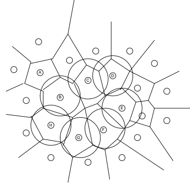
Figure 2. Voronoi diagram of the devices in Fig. 1. The circles represent the coverage disks of the devices that define the inner hole in Fig. 1. Note that the coverage disk of any of these devices does not cover entirely the Voronoi cell of the device.
