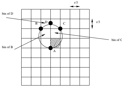
Fig. 9. Proof of Theorem 5.1 – divide the area in r/3 \times r/3 bins. Each bin contains at least one sensor. The hashed bin contains sensor A.
