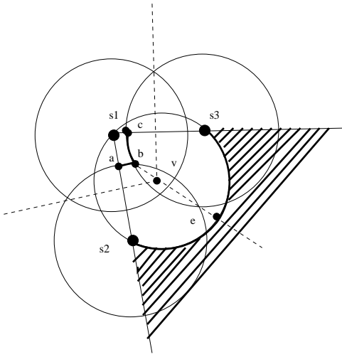
Fig. 3. Proof of Lemma 3.1. If sensors s_1 , s_2 and s_3 are mutual Voronoi generators, another sensor can only be placed in the hashed area. Otherwise, that sensor would be a Voronoi generator of s_1 .
