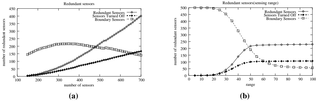
Fig. 10. Plots showing the evolution of the number of boundary sensors, redundant sensors and sensors that can be turned off.
