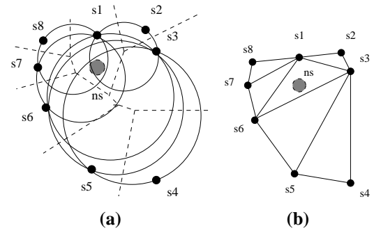
Fig. 6. Example of new sensor deployment: the gray circle, ns , represents the new sensor. (a) The Voronoi diagram of the old sensors. The circles denote circumcircles of Delaunay triangles. (b) The Delaunay triangulation of the old sensors. Sensor s_1 sends a message only to sensors s_2 and s_3 . When sensor s_3 receives the notification from sensor s_2 , it first constructs its list of notifiables, consisting of sensors s_2 , s_4 , s_5 , s_6 , and s_1 . It then colors sensor s_2 gray, since sensor s_2 is the one that sent it the notification. It then traverses the list of notifiables. In the first traversal it colors sensor s_4 gray. We note that this is natural, since we already know that sensor s_2 is closer to sensor s_1 than sensor s_3 . In the next traversal, sensor s_3 colors sensor s_6 gray, since \text{dist}(s_3, s_6) > \text{dist}(s_1, s_6) . The next traversal colors sensor s_5 gray and the last colors sensor s_4 gray. When sensor s_6 receives the notification from sensor s_7 , that received it from sensor s_8 , it constructs its list of notifiables, s_7 , s_1 , s_3 , s_5 . It marks sensor s_7 gray and propagates the gray color to sensors s_1 and s_3 . It then marks sensor s_5 black and notifies it. The notification similarly reaches sensor s_4 .
