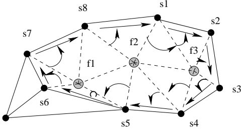
Fig. 8. Example of network in which sensors f_1 , f_2 and f_3 fail simultaneously. The round arrows illustrate the local decisions made by intermediate sensors, and the straight arrows illustrate the trajectory of the DISC messages. Let's say that sensor s_7 detects that f_1 has failed. Sensor s_7 creates a DISC message containing f_1 in the failed list, and sends it to sensor s_8 . Before sending to f_2 , sensor s_8 detects that f_2 has also failed, and adds f_2 to the failed list. Node s_8 then forwards the DISC message to sensor s_1 . Similarly, sensor s_1 adds f_3 to the failed list and forwards the message to sensor s_2 . When sensor s_4 receives this DISC message, it detects that f_2 and f_3 are already in the failed list, so it forwards the message to sensor s_5 , without modifying the failed list. All the intermediate sensors add their identities and positions to the affected list, so when sensor s_7 receives the DISC message that it initiated, it is able to correctly recompute its Voronoi generators and incident Delaunay triangles.
