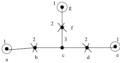
Fig. 5. Example of a redundant graph of a network – the numbers associated with the nodes represent their degree. The circled nodes represent winners in the first round, and the crossed nodes represent their direct neighbors, losers. Node c is not a loser in the first round since none of its neighbors is a winner, but it is a winner in the second round.
