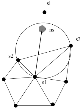
Fig. 7. Illustration of the correctness proof for the join algorithm. ns is the added sensor, s_i is the introducer, s_2 and s_3 are notifiables at Delaunay distance 1 - 1 from s_i , and s_1 is a notifiable at Delaunay distance 1 from s_i .
