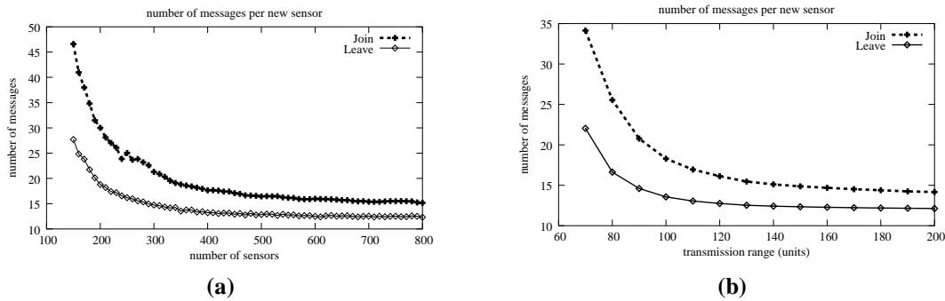
Fig. 11. Plots showing the total number of messages required for the deployment of new sensors.
