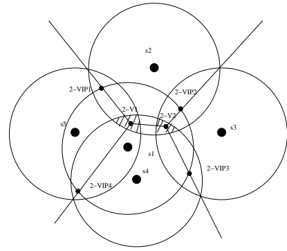
Fig. 4. Example redundant sensor, s_1 . Points 2-V_1 and 2-V_2 are 2-VVs of s_1 , and 2-VIP_{1..4} are 2-Voronoi Intersection Points of s_1 . Note that 2-V_{1,2} and 2-VIP_{1..4} are all covered by at least two of the Voronoi neighbors of s_1 .
